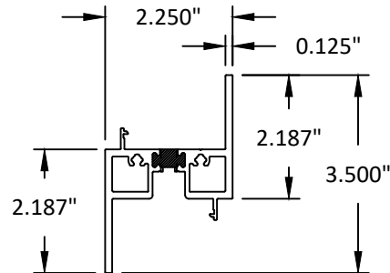
13 MULLION
