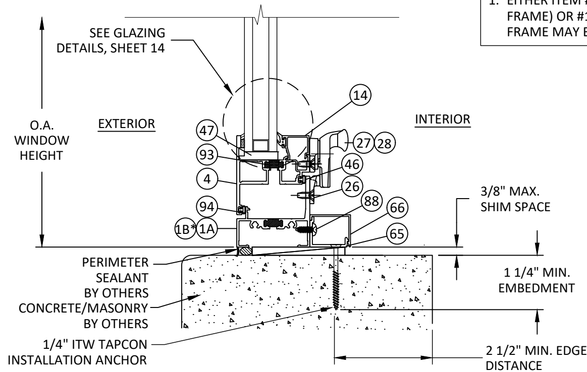
R 10 VERTICAL SECTION VENT SILL - CONCRETE/MASONRY TRIM CLIP ANCHOR - TYP. "OUTSWING"
