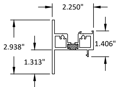
103 MULLION
