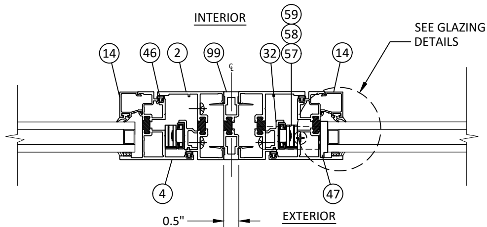
AI 14 HORIZONTAL SECTION "I" MULLION - TYP. PROJECT OUT TO PROJECT OUT
