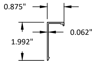
64 ANCHOR CLIP
