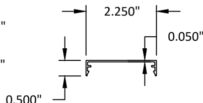
20 COVER
