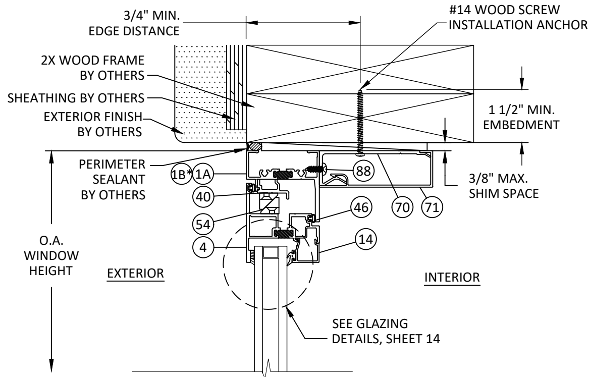
S 10 VERTICAL SECTION VENT HEAD - 2X WOOD FRAME TRIM CLIP ANCHOR - TYP. "OUTSWING"
