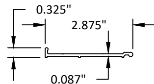
16 SILL TRIM BASE
