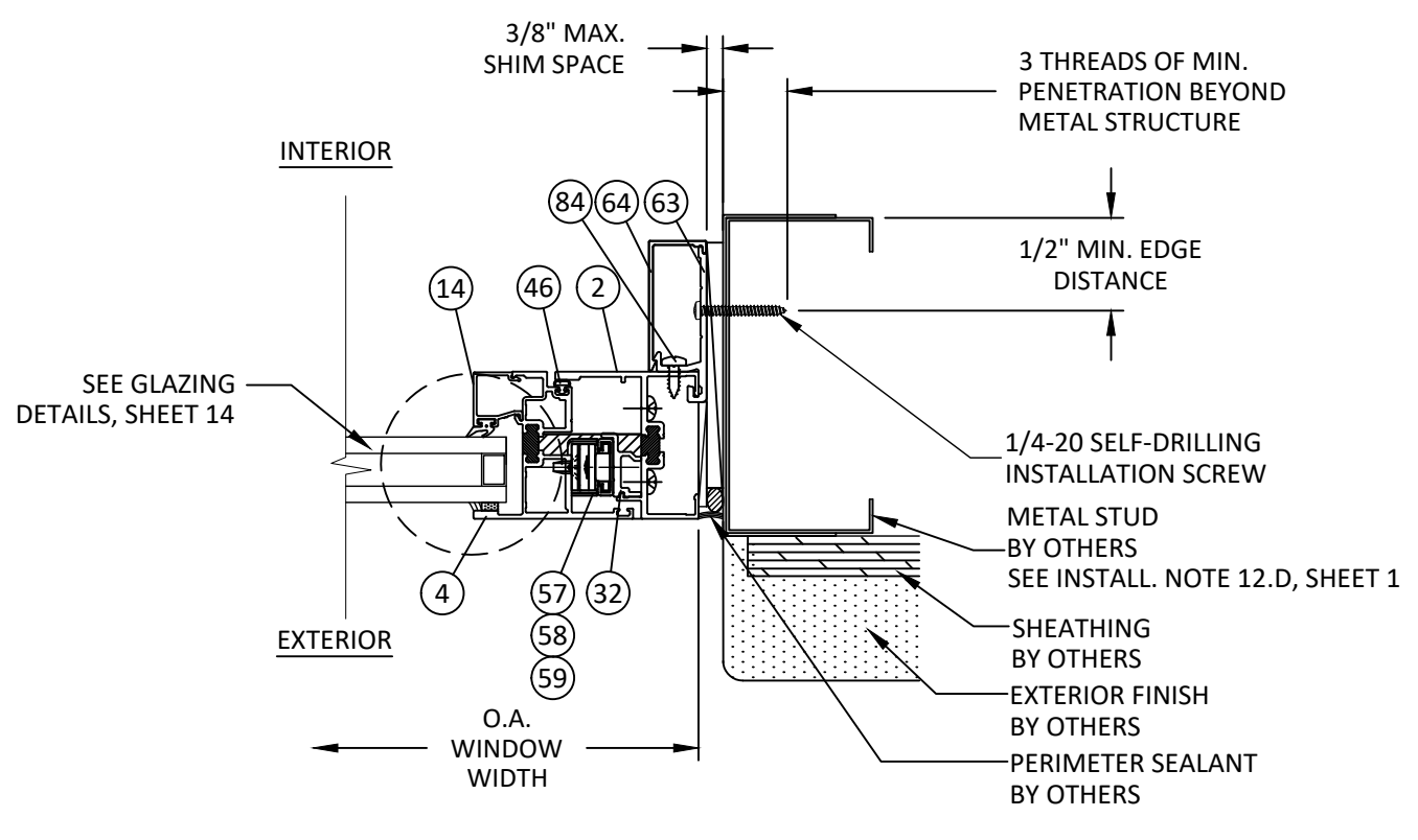
I 7 HORIZONTAL SECTION VENT JAMB - METAL STUD FRAME CLIP ANCHOR - TYP. "OUTSWING"
