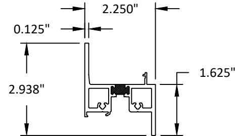
5 MULLION
