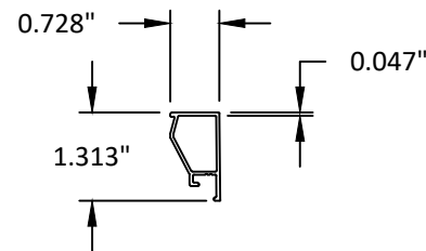
12 FIXED GLASS STOP
