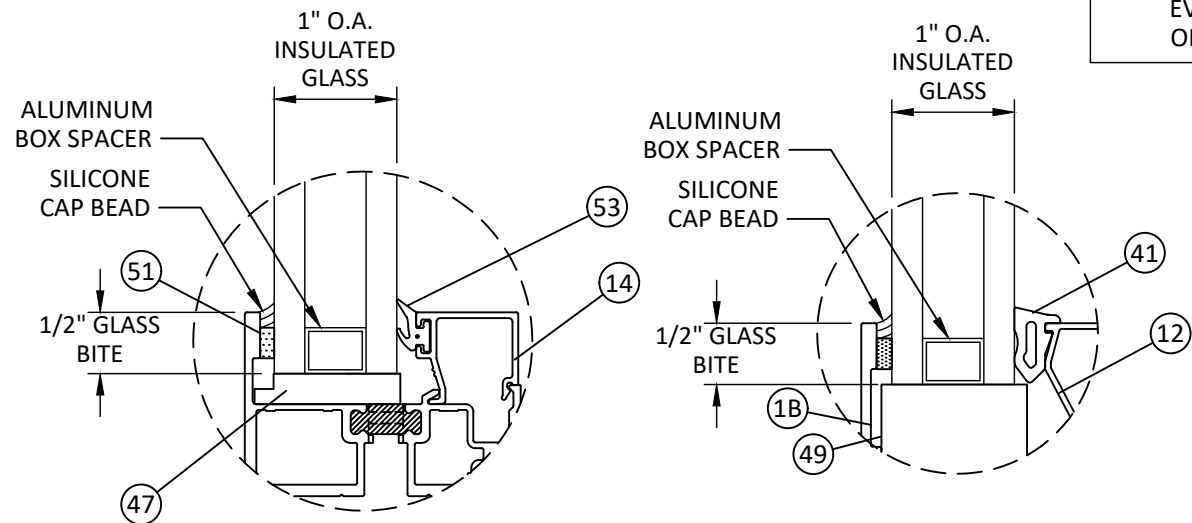
VENT GLAZING DETAILS
