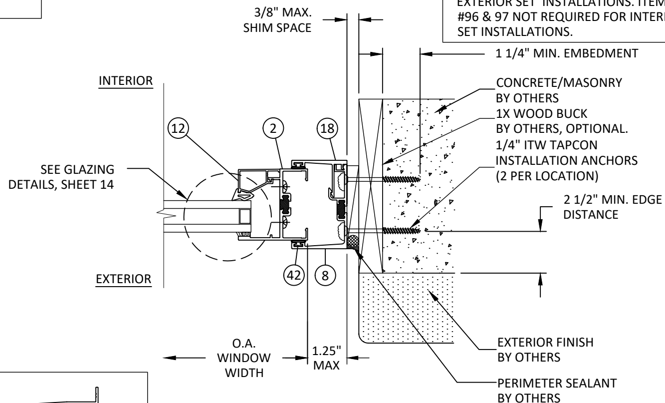
D 6 HORIZONTAL SECTION FIXED JAMB - 1X/CONCRETE/MASONRY INT. SET RECEPTOR - TYP.
