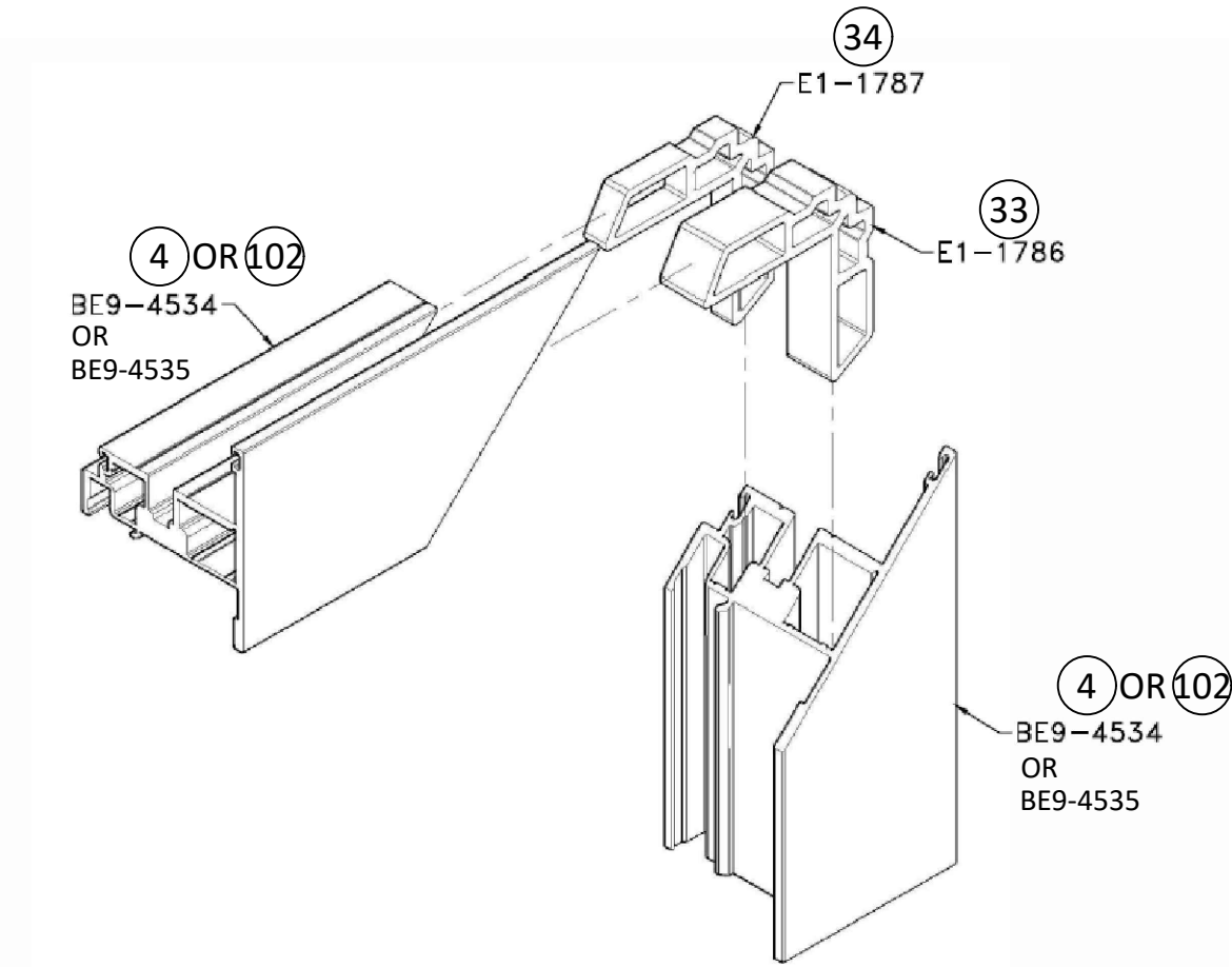
VENT CORNER CONSTRUCTION
