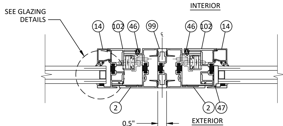
AJ 14 HORIZONTAL SECTION "I" MULLION - TYP. PROJECT IN TO PROJECT IN
