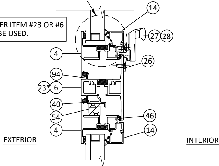
AD HORIZONTAL SECTION 13 PROJECT OUT - PROJECT OUT
