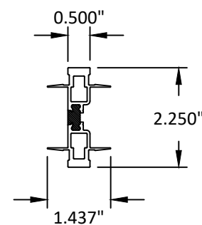
99 I MULLION
