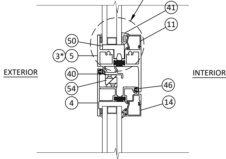
AC VERTICAL SECTION 13 INTEGRAL MULLION-TYP. FIXED OVER PROJECT OUT
