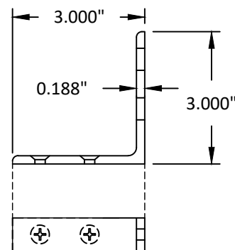
73 MULLION CLIP
