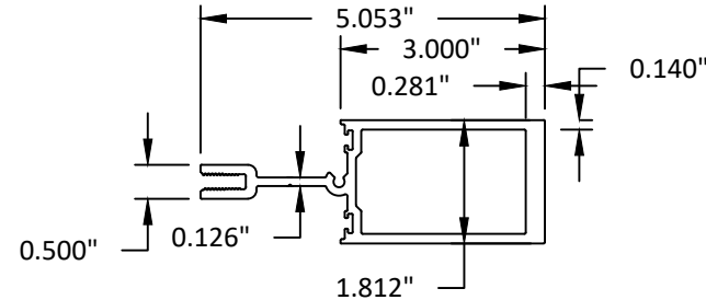
17 STACKING MULLION
