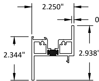
3 MULLION
