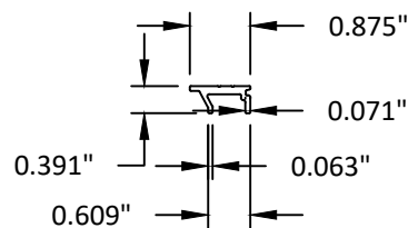
19 LOCK BAR BASE
