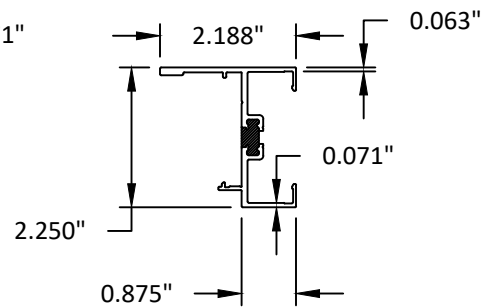
8 RECEPTOR
