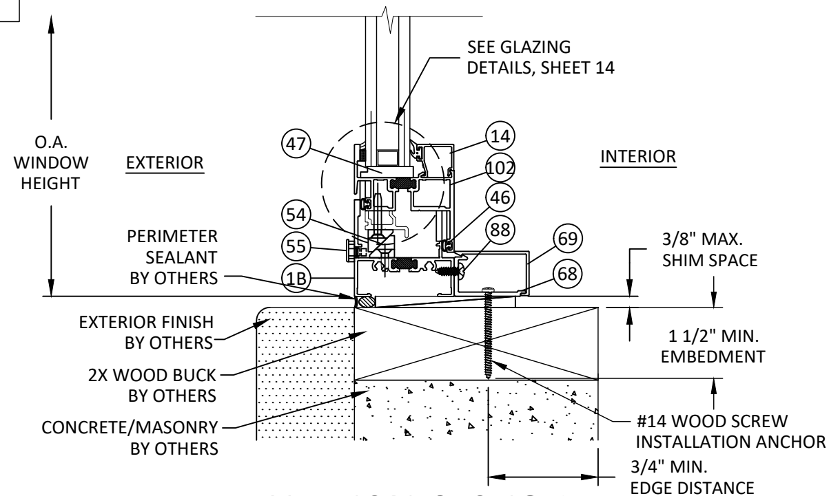
U 10 VERTICAL SECTION VENT SILL - 2X WOOD BUCK TRIM CLIP ANCHOR - TYP. "INSWING"
