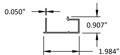
67 STRAP ANCHOR COVER
