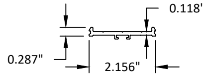
9 PRESSURE BAR
