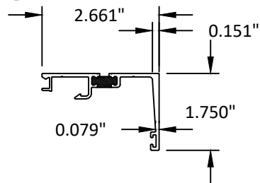
8 RECEPTOR
