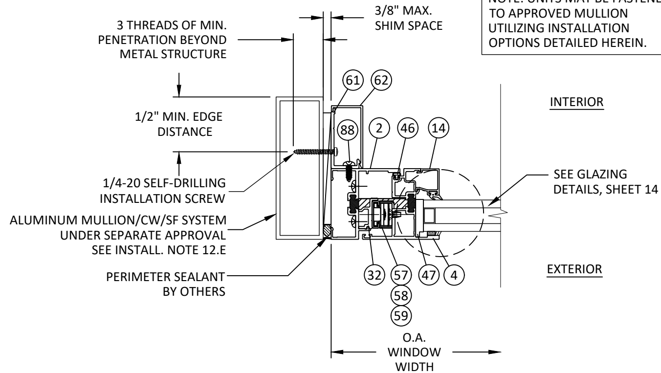
T 10 HORIZONTAL SECTION VENT JAMB - MULL TUBE FRAME TRIM CLIP ANCHOR - TYP. "OUTSWING"
