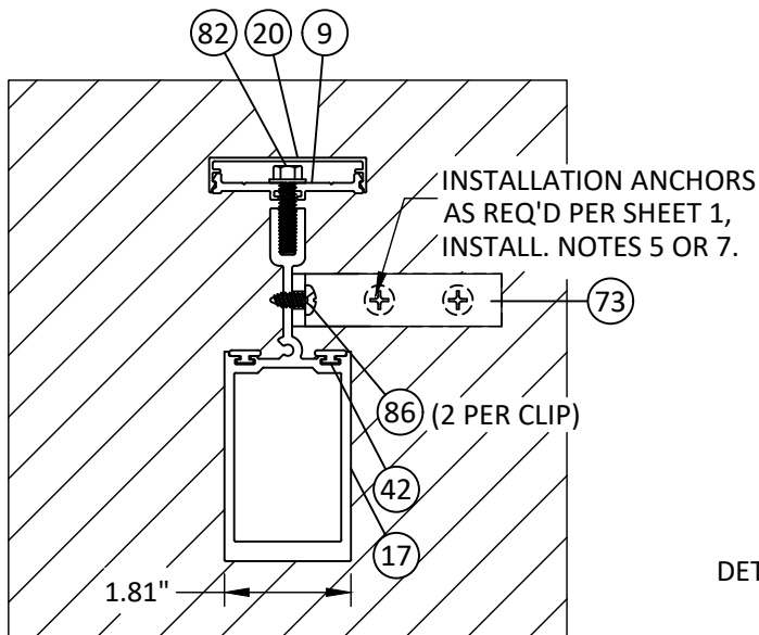
AE HORIZONTAL SECTION 13 STACK MULLION - TYP. JAMB INSTALLATION
