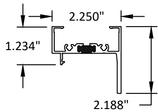
1A FRAME HEAD AND SILL
